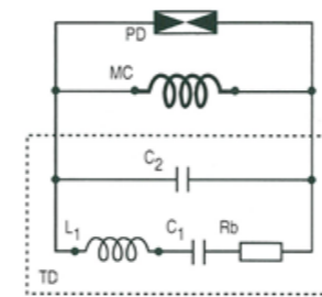
Circuit diagram of a band tuned line trap:
